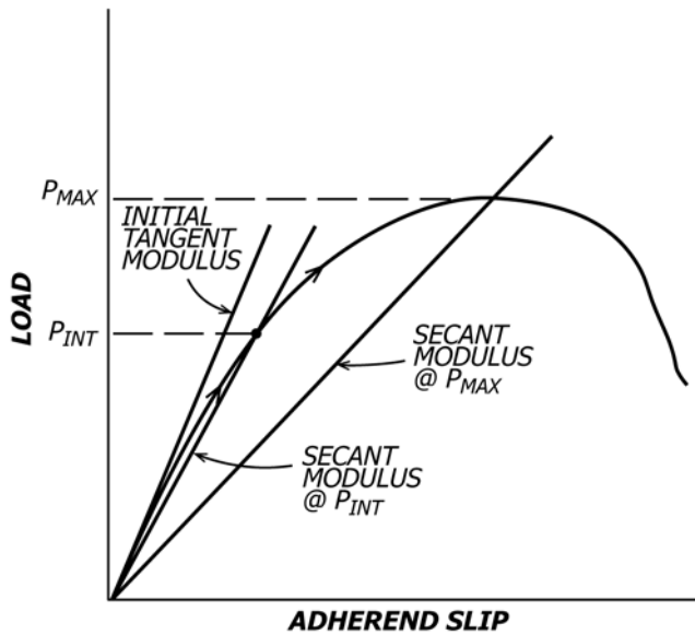
NOTE 1—The modulus may be represented by the initial tangent, the secant drawn to the ultimate load, or the secant drawn to some intermediate load.
